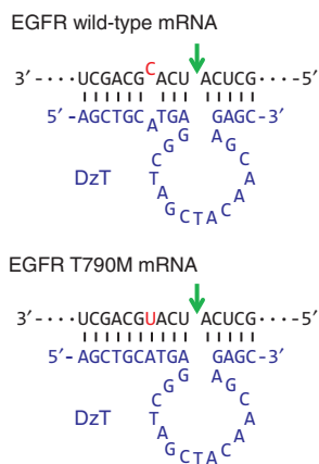
Figure 1 Secondary structure of DzT in complex with EGFR T790M mRNA and wild-type mRNA. The catalytic core of 10–23 DzT (in blue) is flanked by two binding arms with sequences complementary to EGFR T790M mRNA (in black). The sequences of wild-type EGFR mRNA (upper panel) and T790M mRNA (lower panel), RY cleavage site (arrow), and mutation site (in red) are indicated. EGFR, epidermal growth factor receptor; mRNA, messenger RNA.
