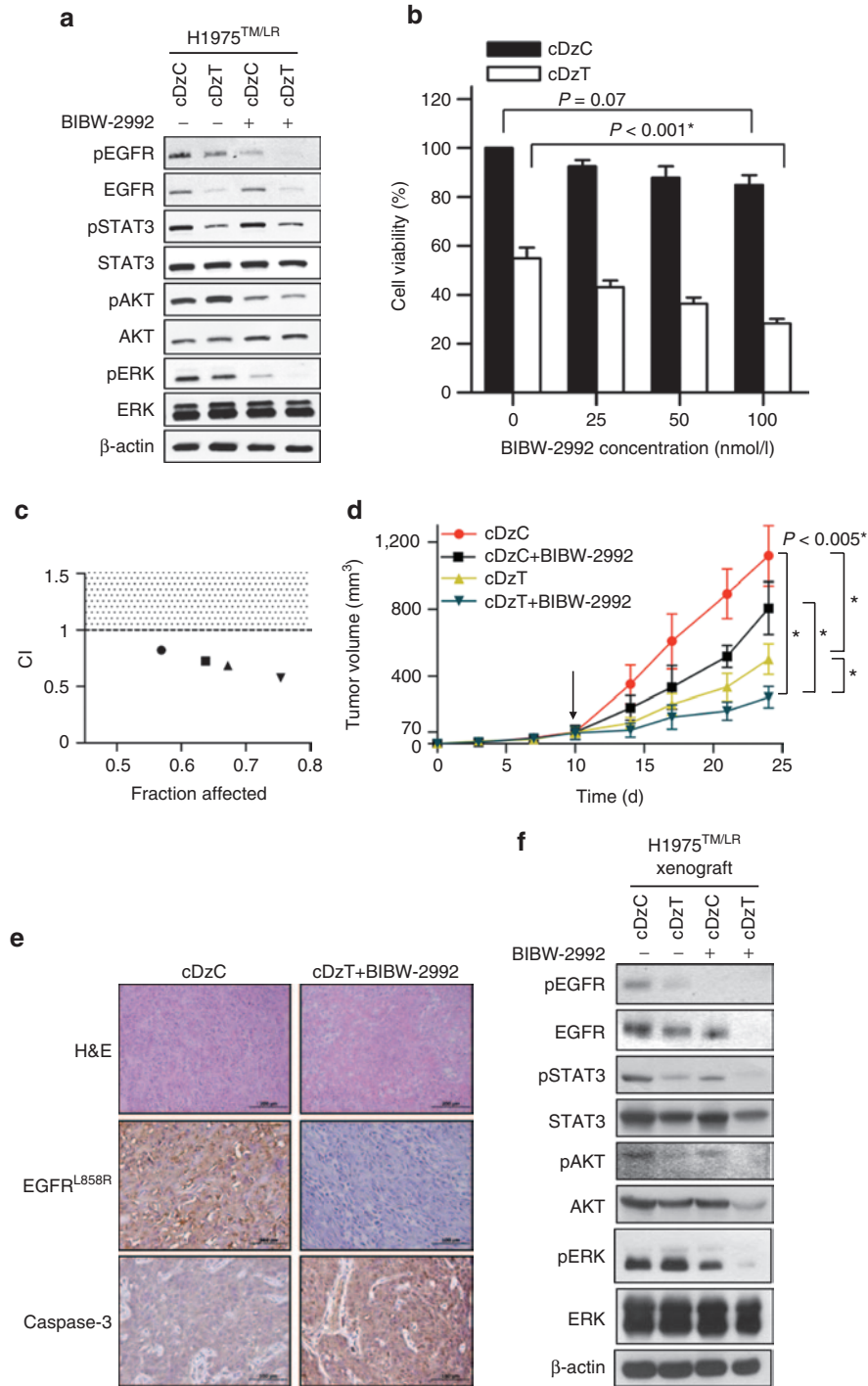
Figure 6 Synergistic effects of cDzT and BIBW-2992. (a) Immunoblot analysis of H1975 TM/RLR cells treated with cDzC or cDzT (50 nmol/l) incubated with or without added BIBW-2992 (200 nmol/l). (b, c) MTT assay of H1975 TM/RLR cells treated with cDzC or cDzT (50 nmol/l) combined with 25 (●), 50 (■), 100 (▲), or 250 nmol/l (▼) BIBW-2992 ( n = 3 ). The data are presented as the mean \pm SD. The results were analyzed by Student's t -test and CI calculation. An asterisk denotes statistical significant difference ( P \leq 0.001 ). (d–f) Combined treatment silences EGFR signaling, triggers apoptosis, and suppresses xenograft tumor growth. (d) cDzT (500 pmoles) was intratumorally injected (twice per week) and BIBW-2992 (20 mg/kg) was orally administrated (three times per week) 10 days (arrow indicated) after inoculating xenograft mice with H1975 TM/RLR ( n = 7 ). The data are presented as mean \pm SD and were analyzed by Student's t -test. Asterisks denote statistical significant differences ( P \leq 0.005 ). (e) Xenograft tumor tissues were processed for immunostaining. Scale bars represent 200 \mu m in H&E images and 100 \mu m in EGFR L858R and caspase-3 images. (f) Xenograft tumor tissues were processed for immunoblotting. CI, combination index; EGFR, epidermal growth factor receptor.
