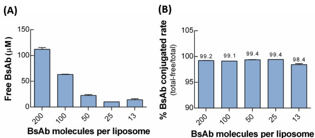
Figure S1. The conjugated rate of the \alpha\text{HER2}/\text{PLD} . (A) The different amount of BsAb mixed with \alpha\text{HER2}/\text{PLD} . After 5 min incubation, the \alpha\text{HER2}/\text{PLDs} were added in mPEG/BSA-coated 96-well plate, and then the free BsAb (unbound) was detected by ELISA using HRP-conjugated anti-human Fab antibody. (B) The conjugated rate of \alpha\text{HER2}/\text{PLD} were calculated by total number of BsAb minus number of free BsAb then divide by number of total BsAb. Results show the mean absorbance values ( n=3 ). Bar, SD.
